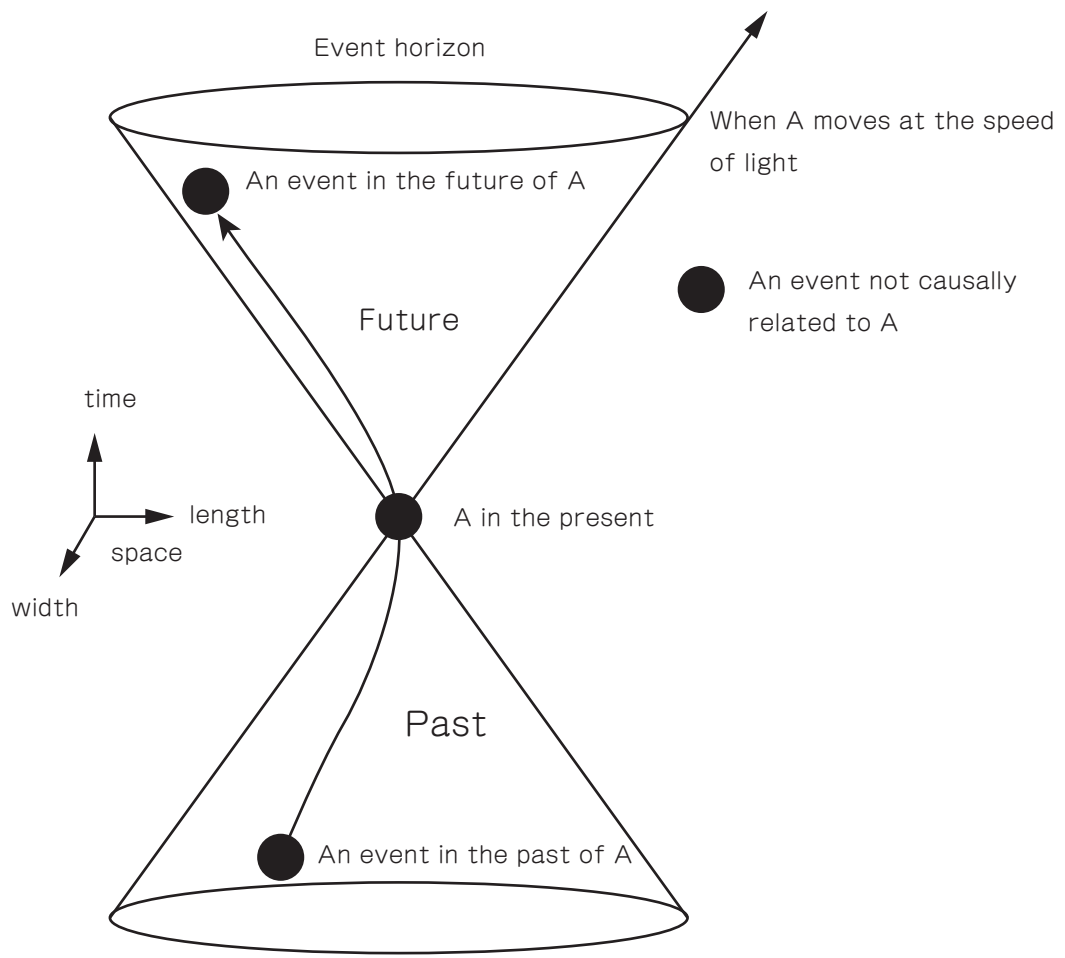
A Minkowski Light Cone
